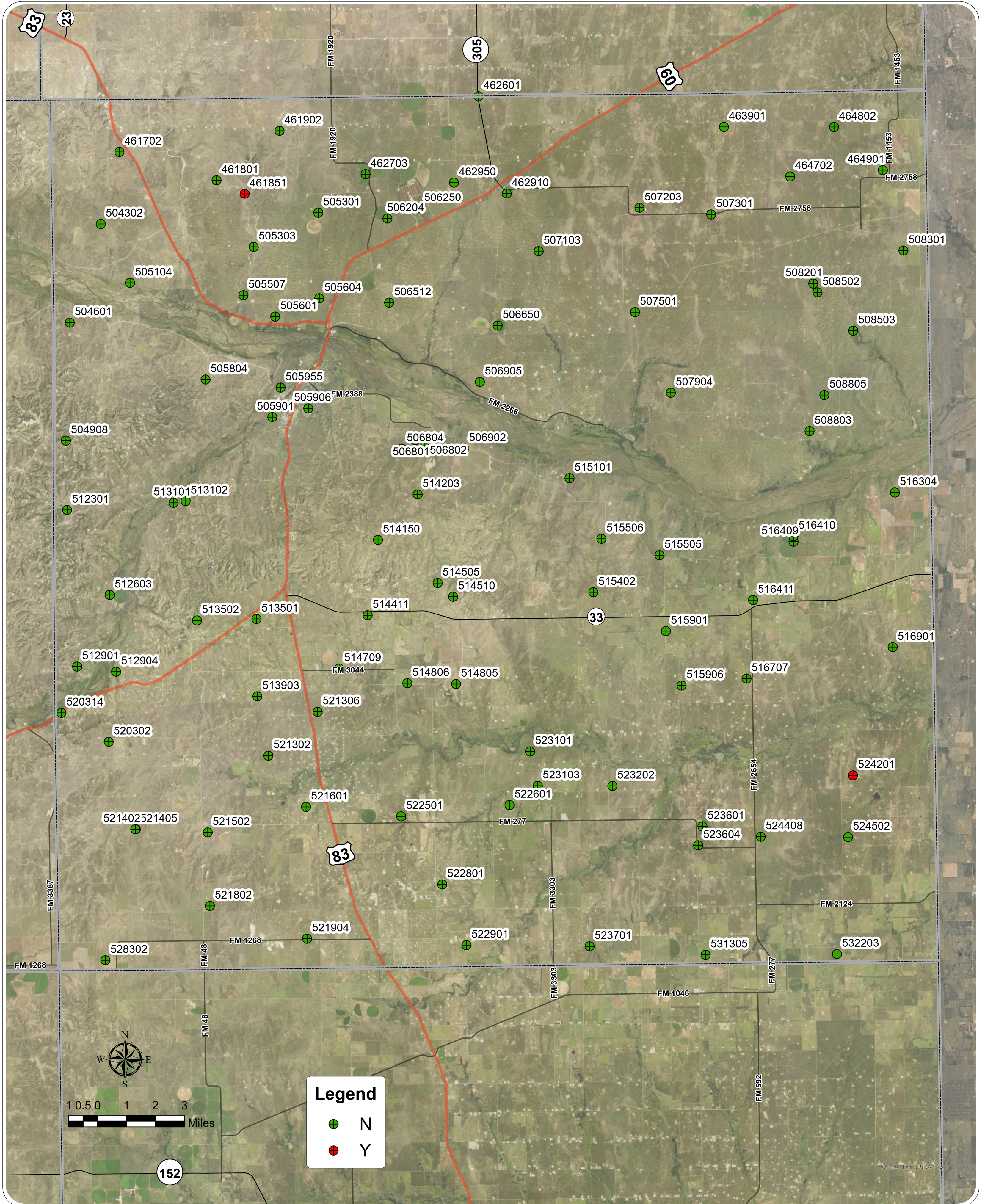
Figure 2 Wells Exceeding Annual Decline Rate FY24-FY25 Hemphill County, Texas
